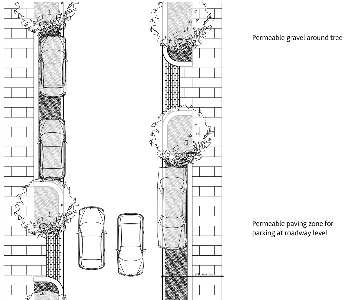
Plan view of street with permeable parking zone
