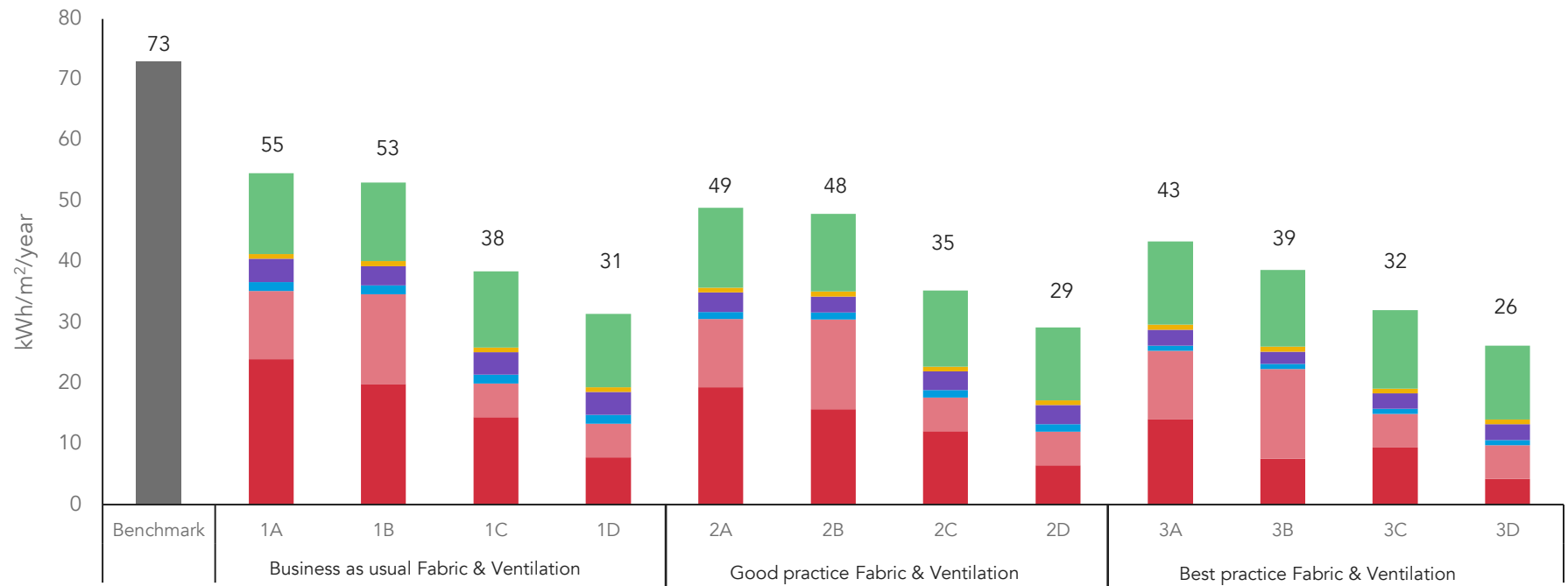
Figure 7.3 - Predictive energy modelling results: bar chart showing the detailed breakdown of energy use intensity (EUI) for each case
