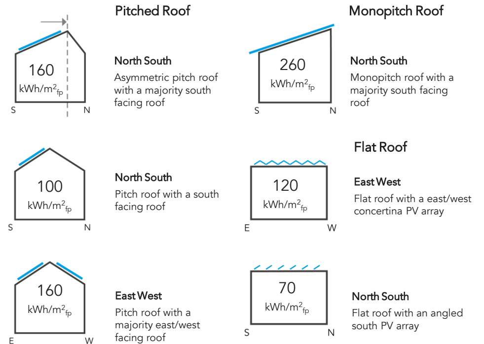
Figure 11.13 - Roof design can be optimised to maximise energy output from photovoltaics. A useful indicator of this is expressed in kWh generated per m 2 of building footprint ( \text{kWh/m}^2_{\text{fp}} )
