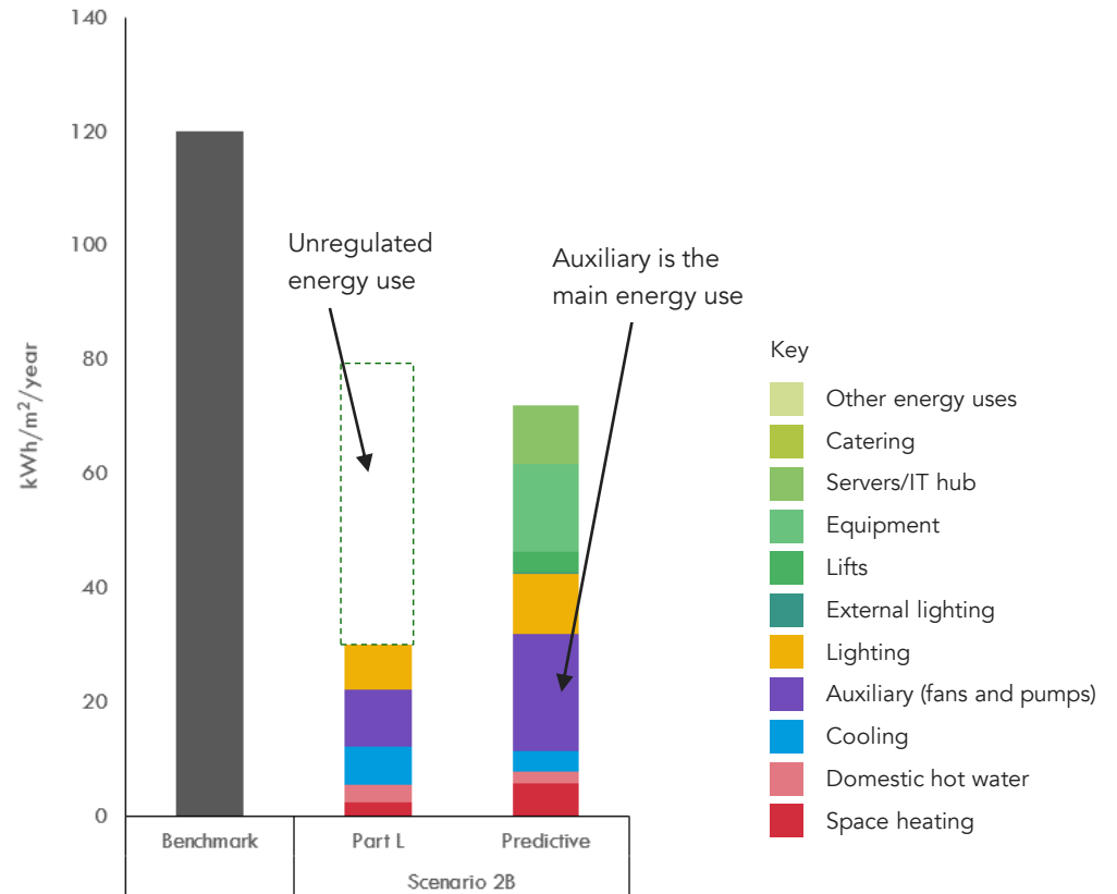
Figure 8.5 – Comparison between the results of the Part L energy model and the Predictive energy model, per separable energy use, for a typical 'good practice' scenario with a heat pump
