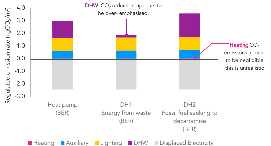
Figure 6.8 - Analysis of district heating and communal heat pump scenarios. Modelling results from each district heating option compared with the 'heat pump-more efficient' scenario
